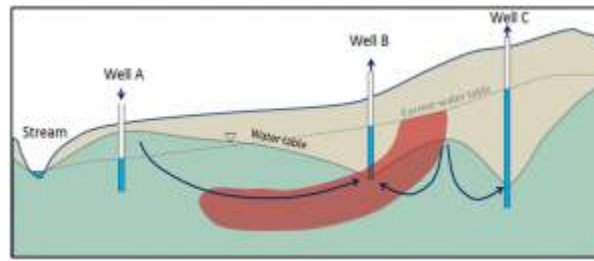
Implications of pumping water from wells B and C and injecting water into well A [SE]
