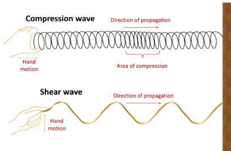
Figure 9.4 A compression wave can be illustrated by a spring (like a Slinky) that is given a sharp push at one end. A shear wave can be illustrated by a rope that is given a quick flick. [SE]
