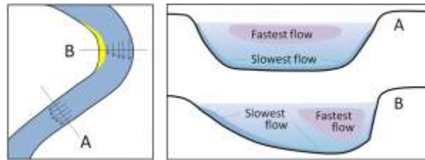
Figure 13.14 The relative velocity of stream flow depending on whether the stream channel is straight or curved (left), and with respect to the water depth (right). [SE]
