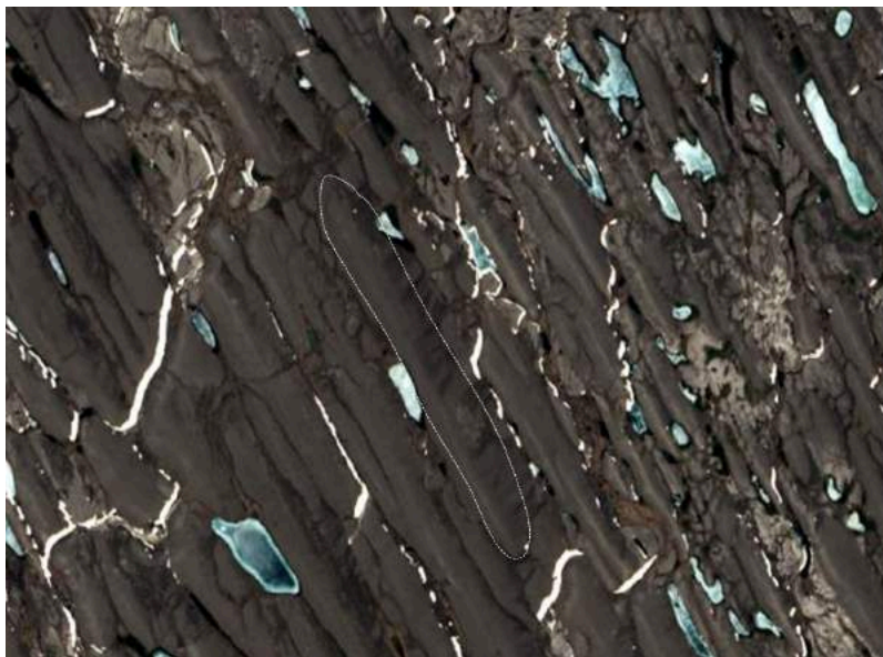
Figure 16.19 Drumlins — streamlined hills formed beneath a glacier, here made up of sediment — in the Amundsen Gulf region of Nunavut. The drumlins are tens of metres high, a few hundred metres across, and a few kilometres long. One of them is highlighted with a dashed white line. [http://earthobservatory.nasa.gov/IOTD/view.php?id=85506]
