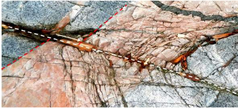
Figure 12.12 A fault (white dashed line) in intrusive rocks on Quadra Island, B.C. The pink dyke has been offset by the fault and the extent of the offset is shown by the white arrow (approximately 10 cm). Because the far side of the fault has moved to the right, this is a right-lateral fault. If the photo were taken from the other side, the fault would still appear to have a right-lateral offset. [SE]
