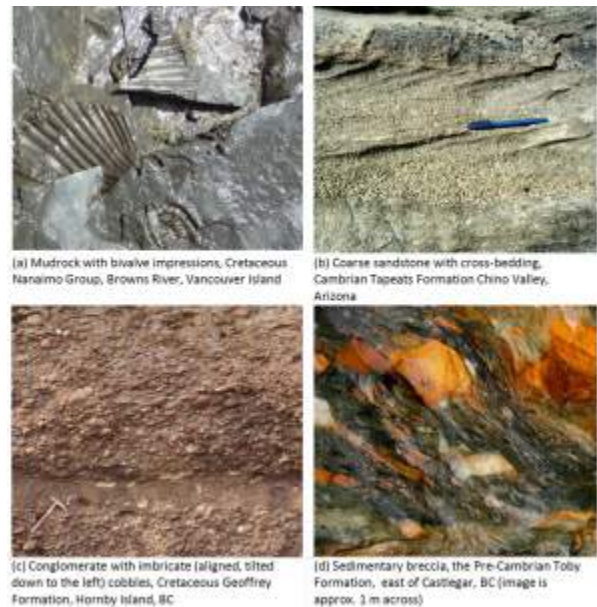
Figure 6.8 Examples of various clastic sedimentary rocks.
