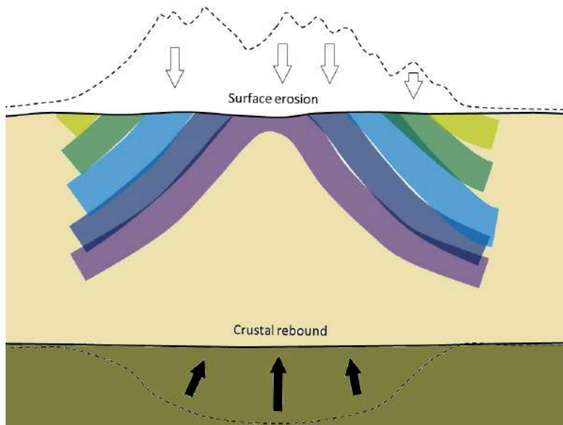
Figure 7.23 (b) Schematic present-day cross-section through the Meguma Terrane.
