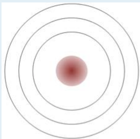
Chlorine (17)
