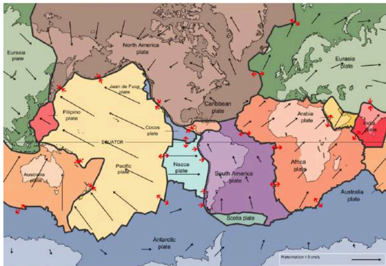
Figure 10.16 A map showing 15 of the Earth's tectonic plates and the approximate rates and directions of plate motions. [SE after USGS, http://en.wikipedia.org/wiki/Plate_tectonics#/media/File:Plates_tect2_en.svg ]
