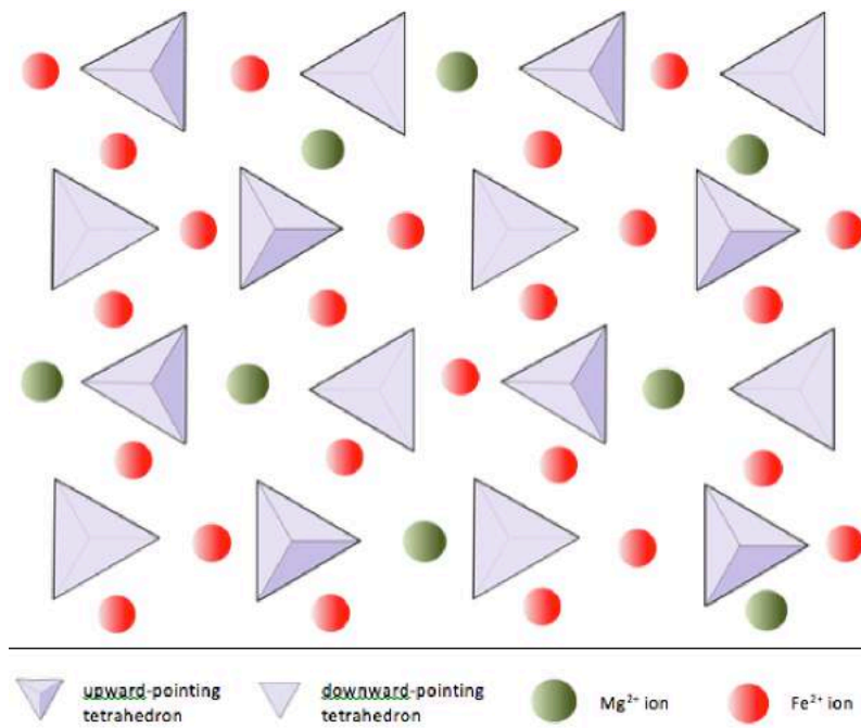
Figure 2.10 A depiction of the structure of olivine as seen from above. The formula for this particular olivine, which has three Fe ions for each Mg ion, could be written: \text{Mg}_{0.5}\text{Fe}_{1.5}\text{SiO}_4 .
