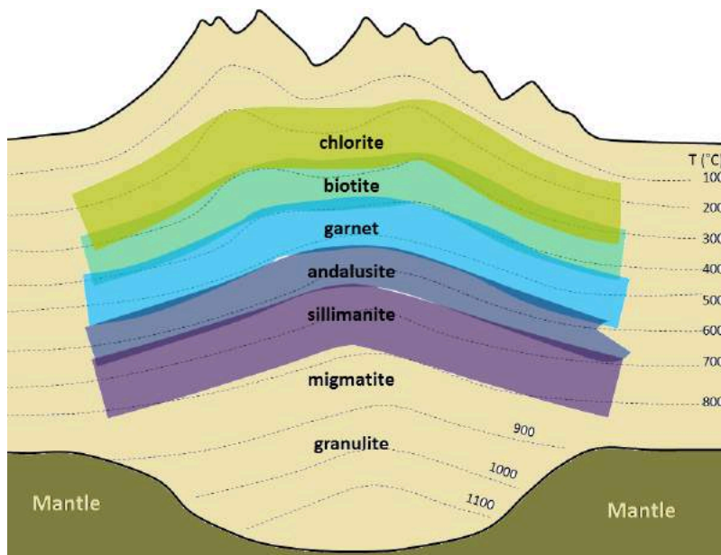
Figure 7.23 (a) Schematic cross-section through the Meguma Terrane during the Devonian.
