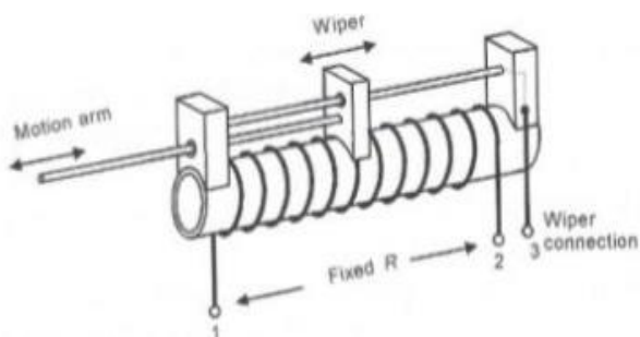
Fig.10. Potentiometric displacement sensor
