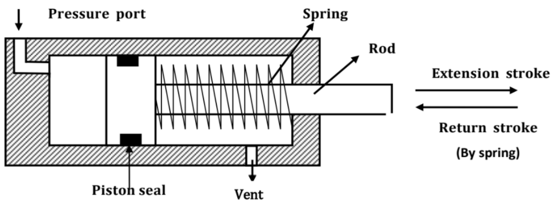
Fig 1. Construction features of single acting cylinder
