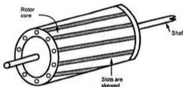
Fig.19. Squirrel cage Induction Motor
