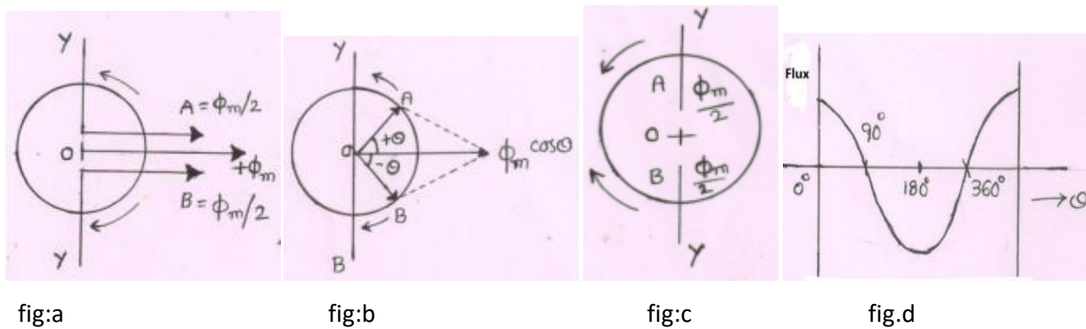
Fig.22. Double revolving field theory
