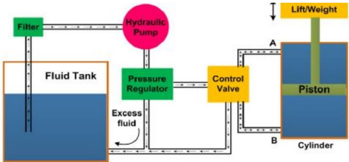
Fig.5. Schematic of Hydraulic system
