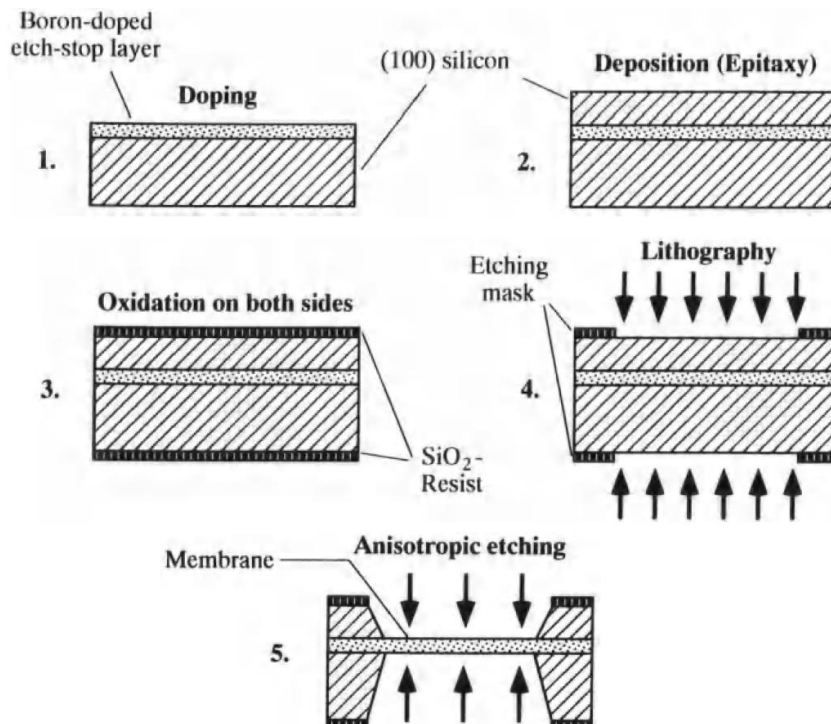
Fig.10. The production of a membrane by the p+ etch-stop technique
