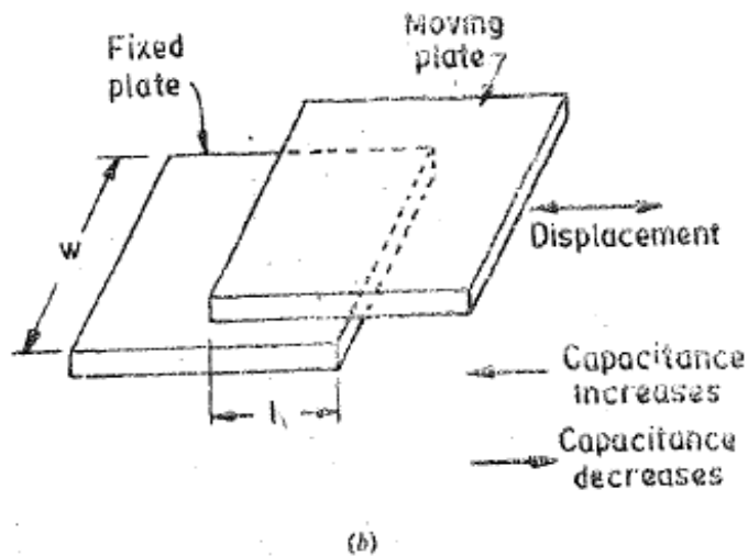
Fig.20. Capacitive transducer using change of area principle
