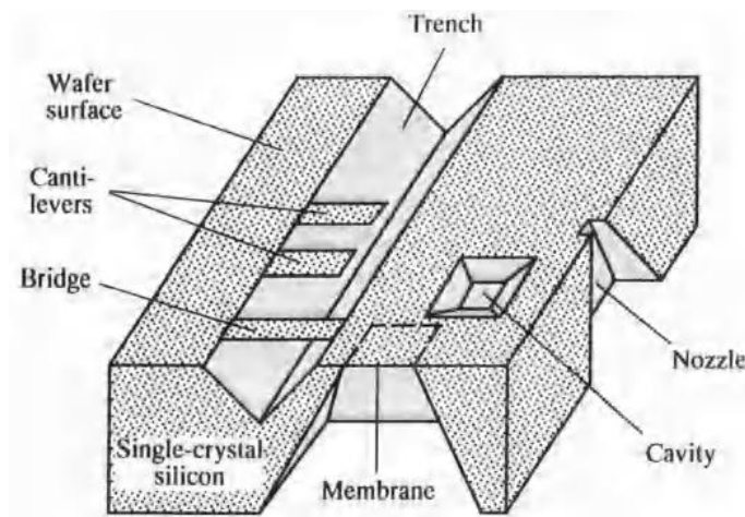
Fig.9. Various bulk micromachining structures.
