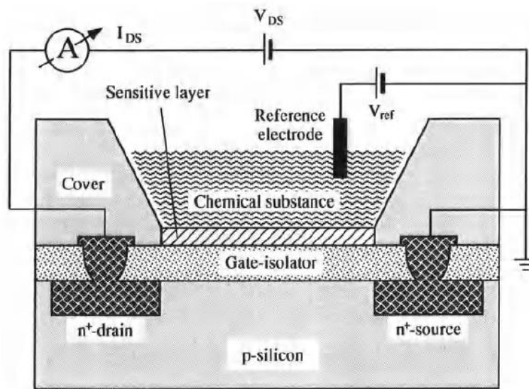
Fig.10. Chemical sensor
