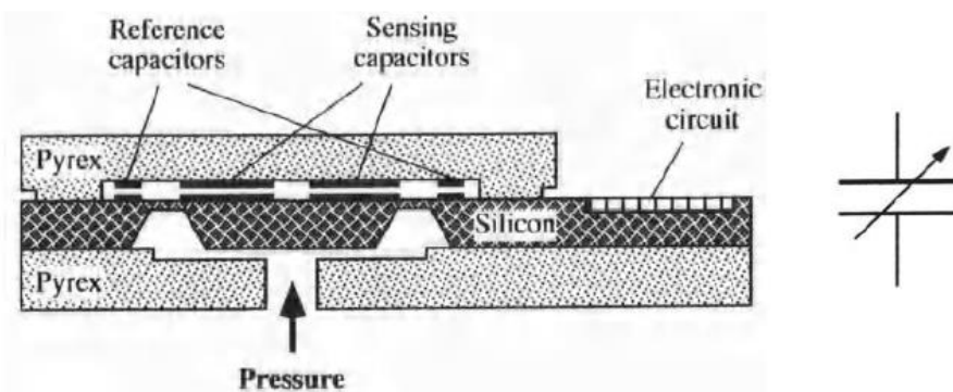
Fig.2. Capacitive pressure sensors
