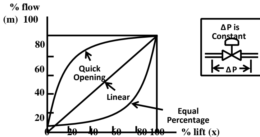
Fig. 13 Flow characteristics of control valves
