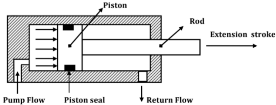
Fig.6. Double acting cylinder
