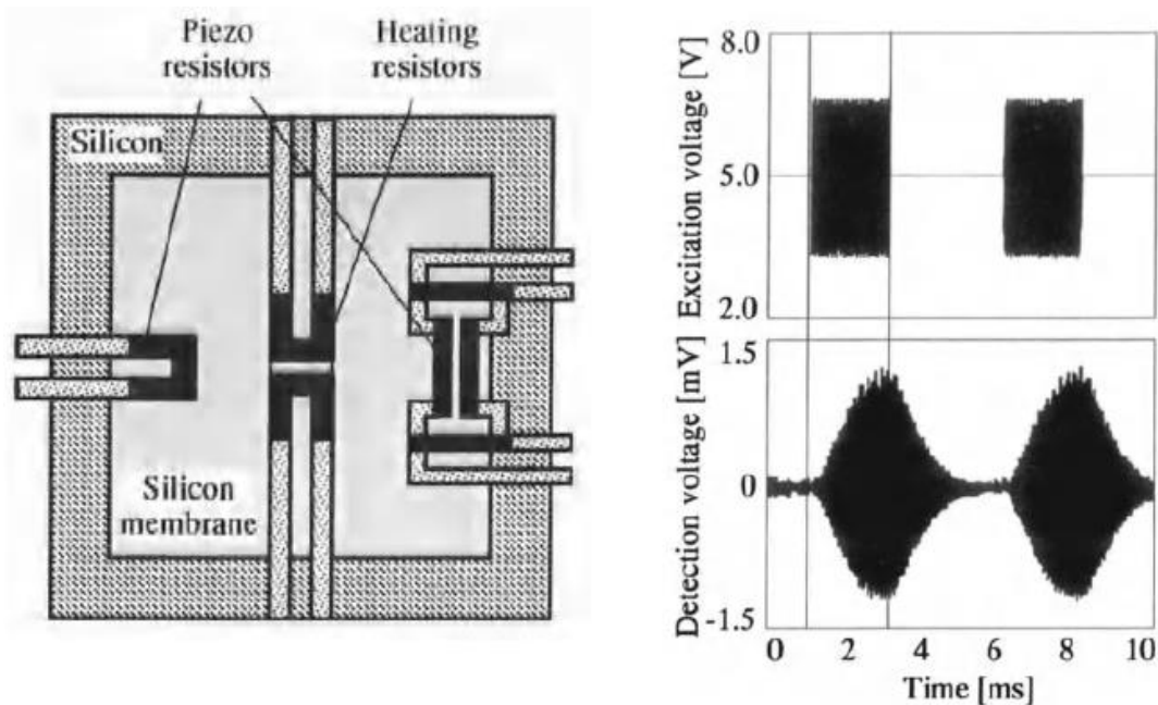
Fig. 4. Ultrasound distance micro sensor
