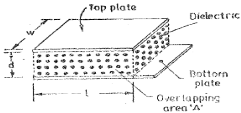
Fig.19.Schematic diagram of parallel plate capacitor
