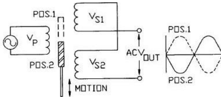
Fig. 8. Working of LVDT
