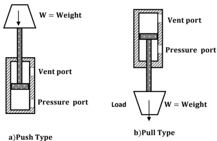
Fig 4. Gravity return type single acting cylinders
