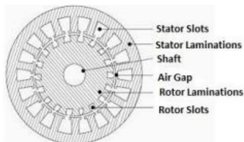
Fig. 21. Single phase induction motor
