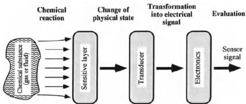
Fig.9. General Structure of chemical sensors
