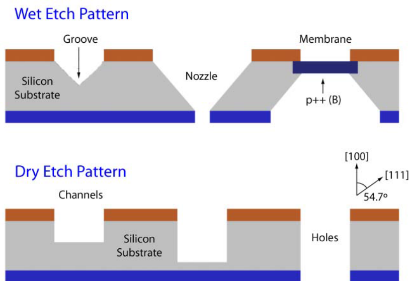
Fig.12. Wet and Dry etch techniques
