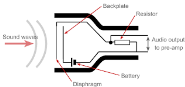
Fig.24._capacitor / condenser microphone
