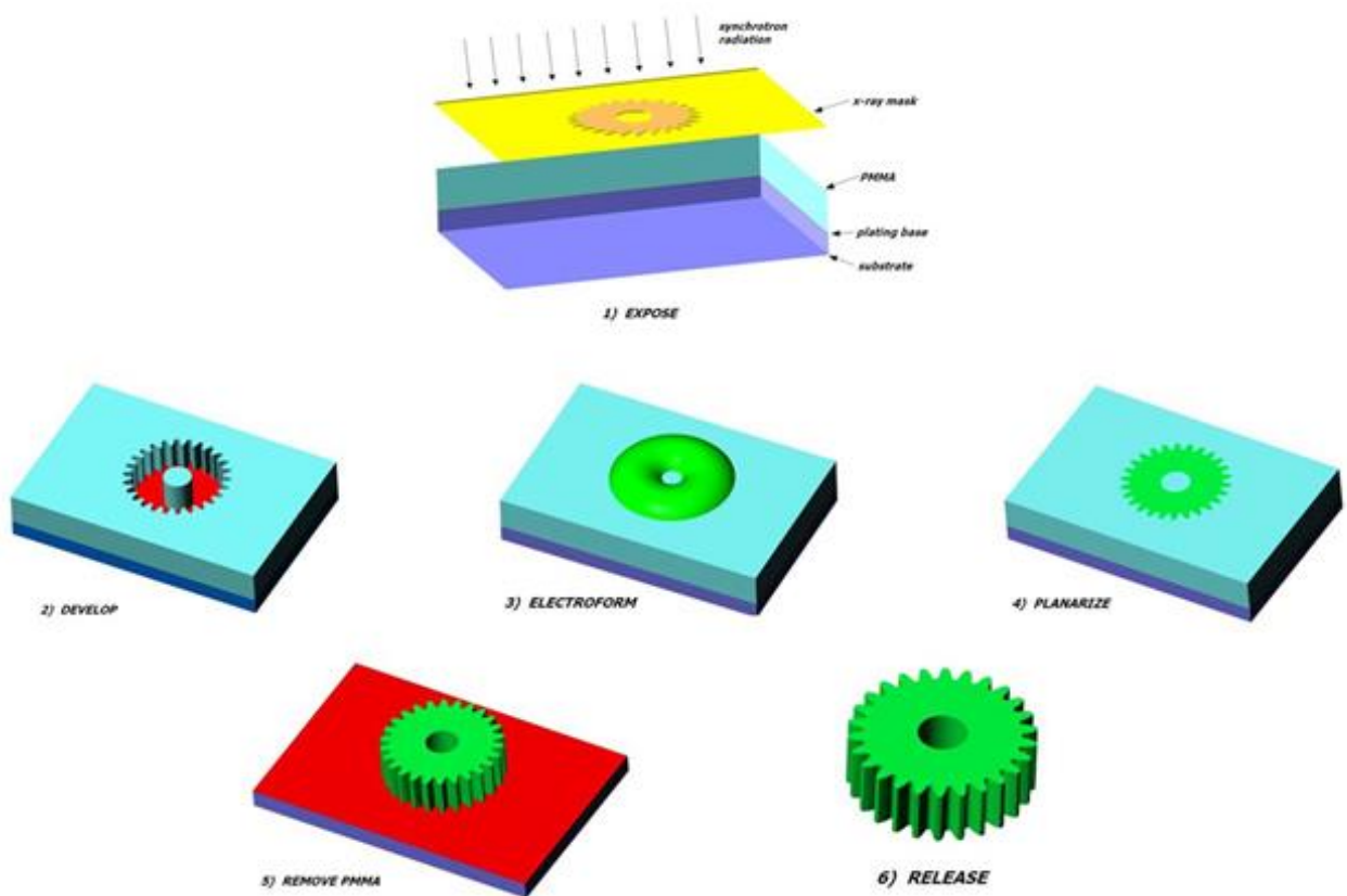
Fig.20. Full LIGA process
