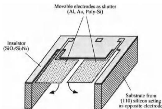
Fig.4. Electrostatic micro shutter
