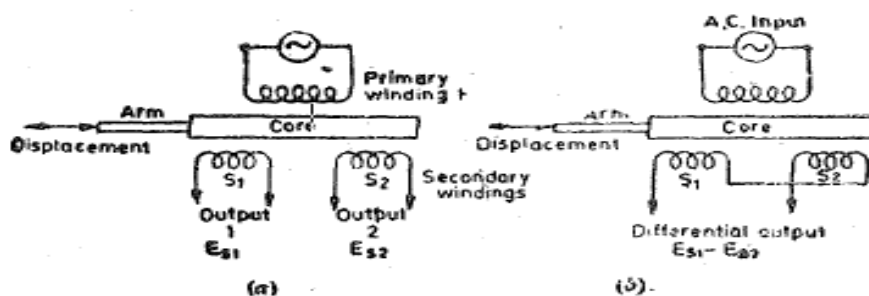
Fig. 2. Circuits of an LVDT
