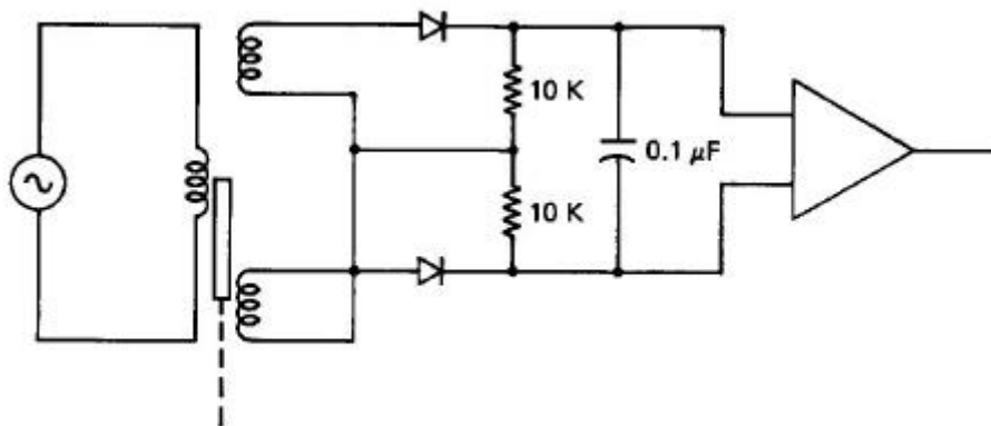
Fig.9. LVDT circuit
