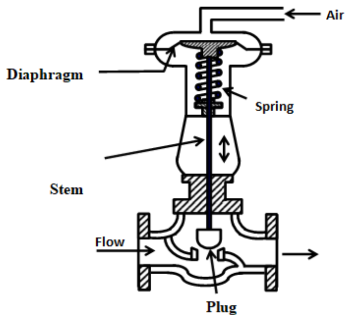
Fig. 10 Control valve
