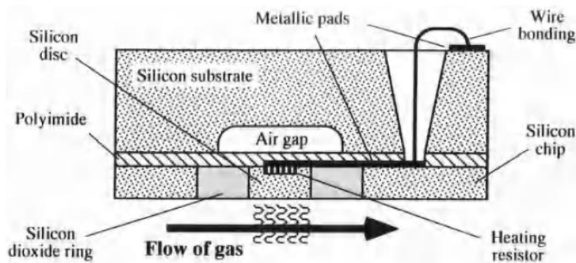
Fig.15. Thermal flow sensor
