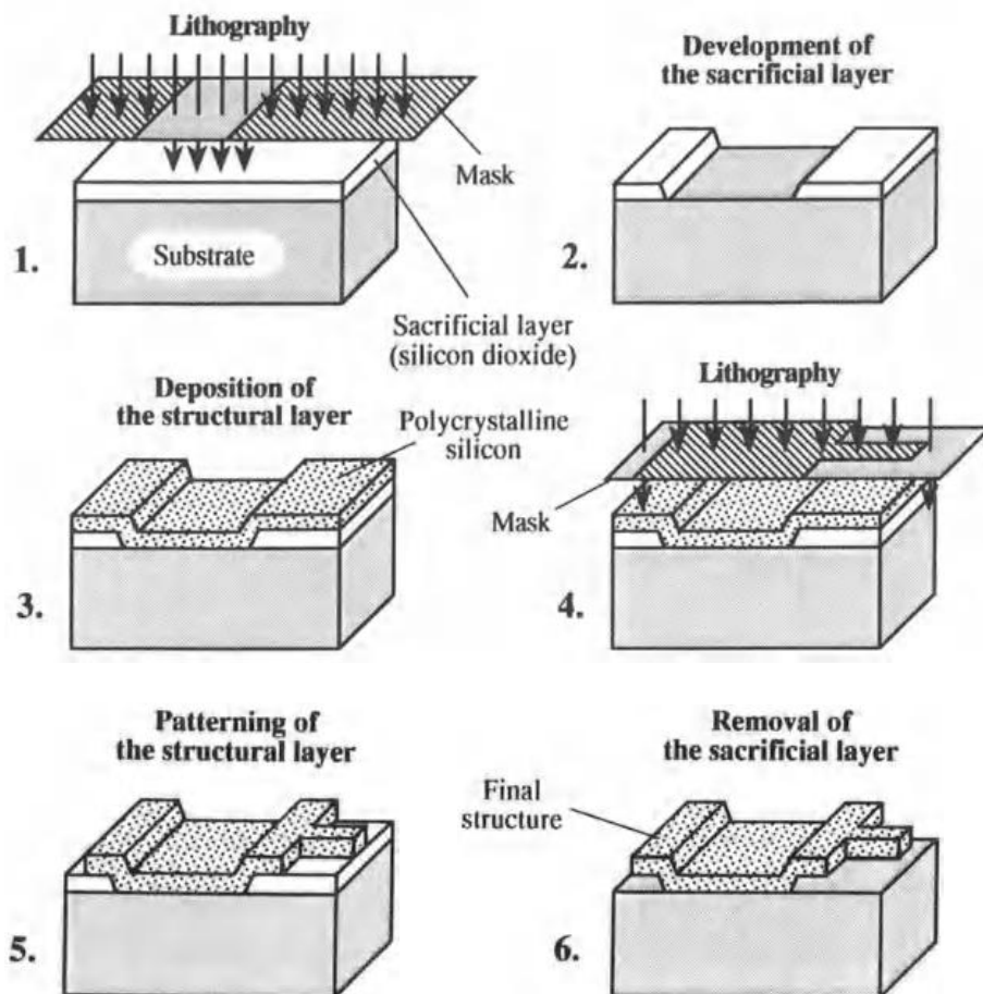
Fig.15. Processing steps of surface micromachining.
