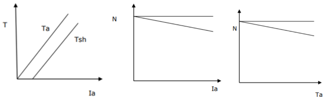
Fig.7. Shunt motor Characteristics
