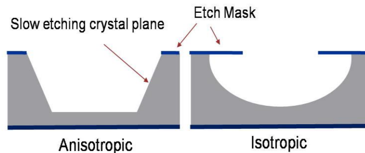
Fig.13. Anisotropic and Isotropic etch
