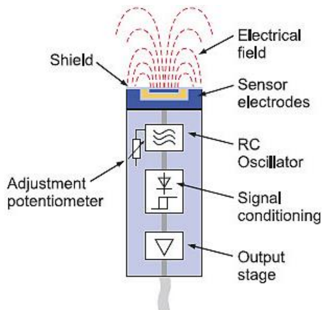
Fig.29. Capacitive proximty sensor
