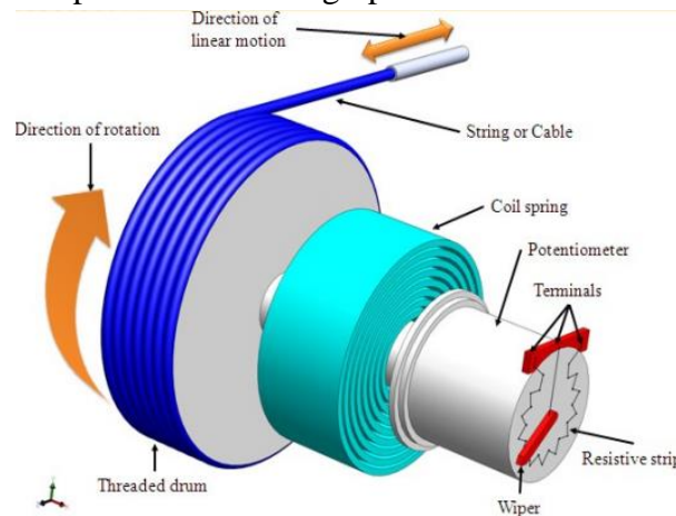
Fig.11. Schematic of a rotary type potentiometer sensor for measurement of linear displacement
