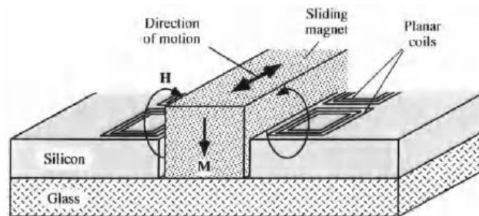
Fig.8.Linear micro motor
