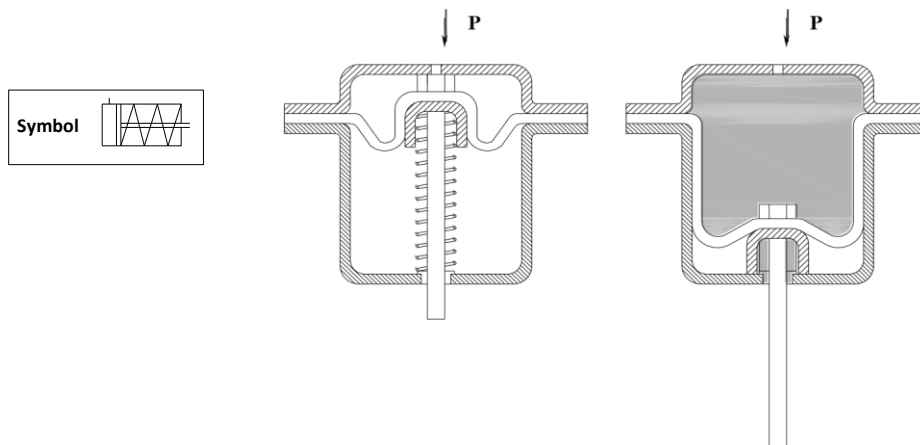
Fig 3 Construction features of rolling diaphragm cylinder
