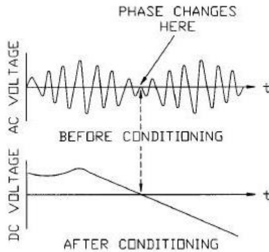
Fig.10. Signal conditioning waveforms.
