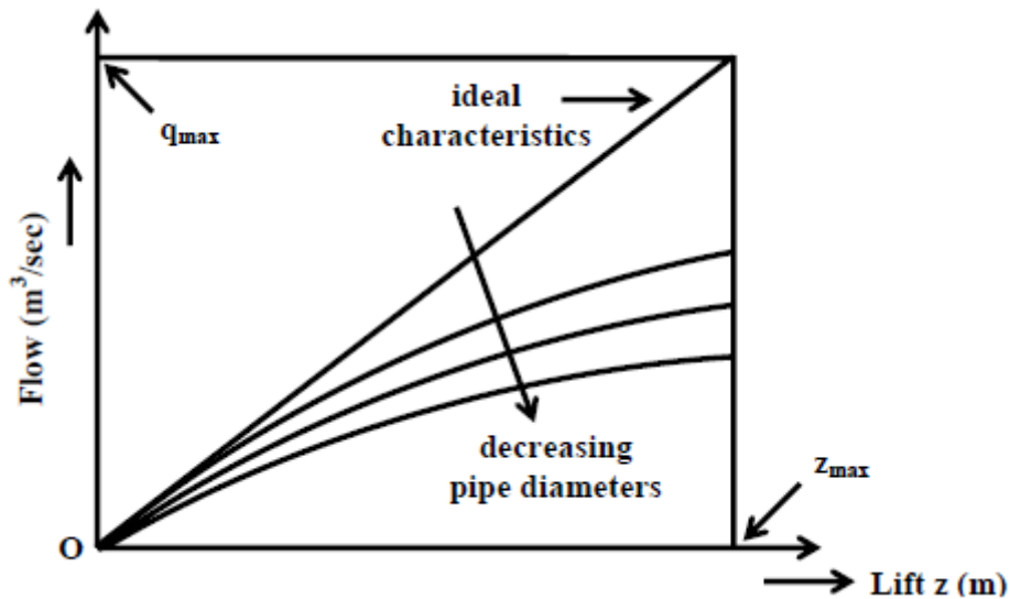
Fig. 16. Effect of pipeline diameter on the effective flow characteristics the control valve
