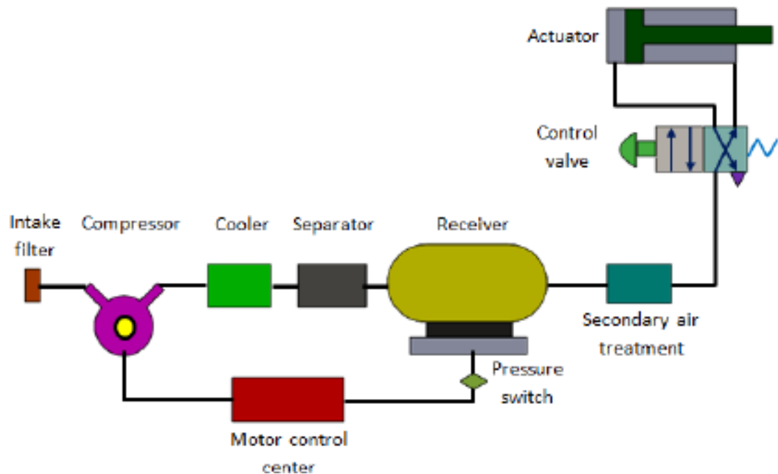
Fig. 6. Schematic of Pneumatic system
