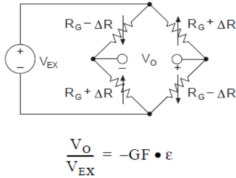
Fig. 18. Full bridge circuit
