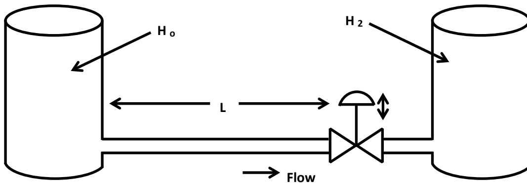
Fig.15. Effect of friction loss in pipeline for a control valve
