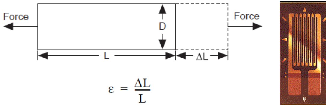
Fig. 14. strain gauge
