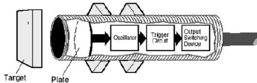
Fig.28. Capacitive proximty sensor
