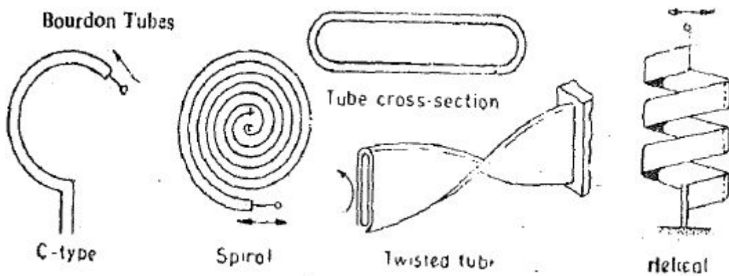
Fig. 7. Types of Bourdon tubes
