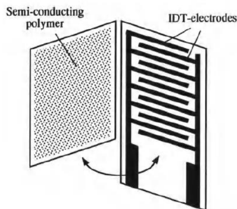
Fig. 3. A force sensing resistor
