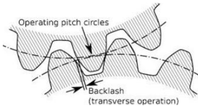
Fig. 4. Backlash
