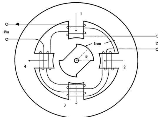
Fig.17. Microsyn
