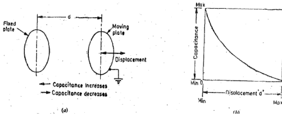
Fig.21. Capacitive transducer using change of distance between plates principle
