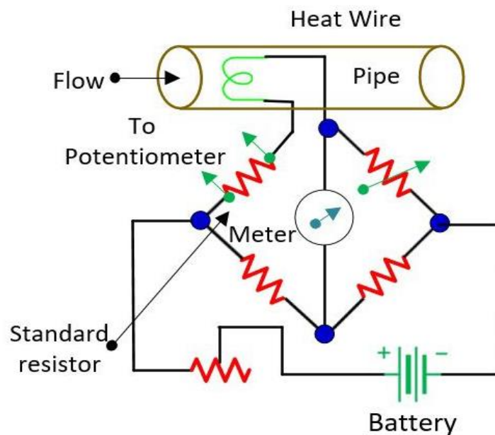
Fig. 27. Measurement of fluid flow
