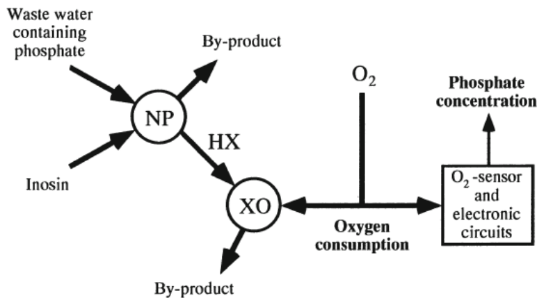
Fig.11 Phosphate measurement with metabolism sensor
