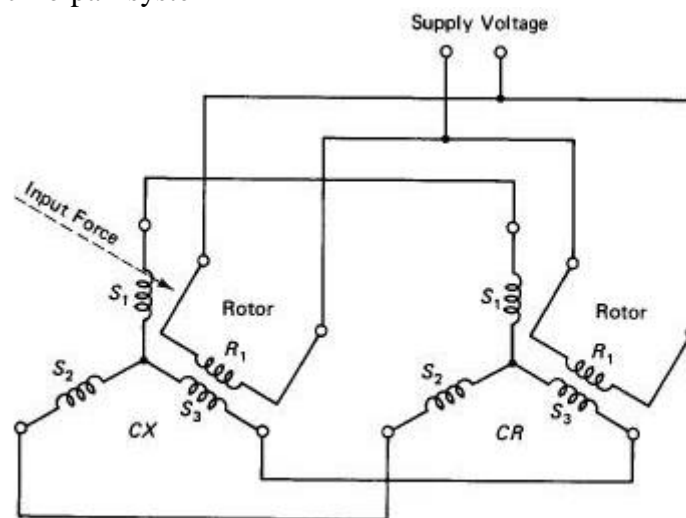
Fig.15.TX -RX synchros in controlling positioning of an antenna
