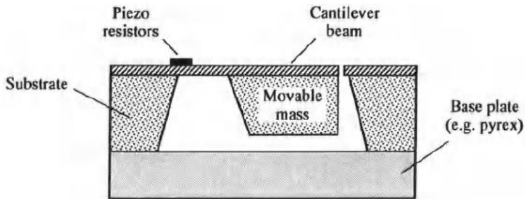
Fig.7 Piezo resistive principle for acceleration measurement
