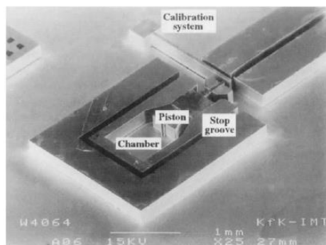
Fig.13. Hydraulic piston micro actuator
