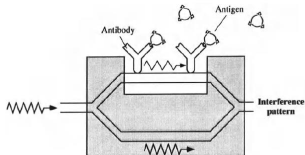
Fig. 12. Immuno sensing using an optical transducer
