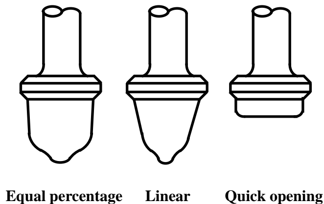
Fig. 14. Valve plug shapes for the three common flow characteristics.
