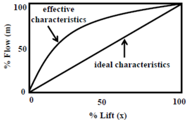
Fig.17. Comparison of ideal and effective characteristics for a linear valve
