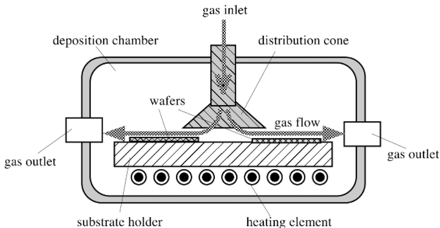
Fig.6. Simplified structure of a CVD reactor chamber.
