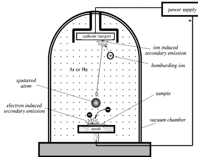
Fig. 5. Sputtering process in a vacuum chamber.
