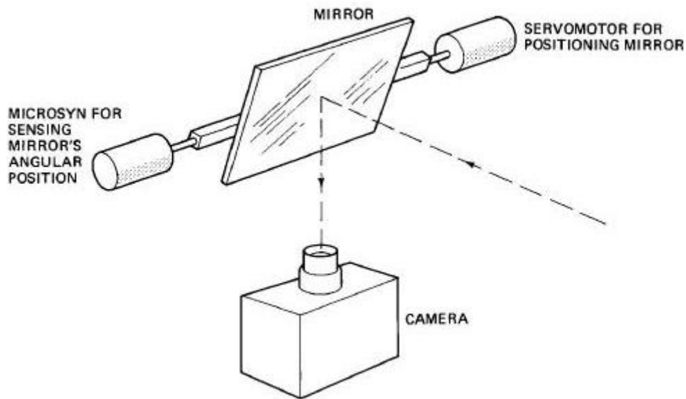
Fig.18. Microsyn application
