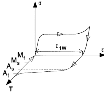
Fig.1 Stress- Strain – temperature characteristic for the one-way effect
