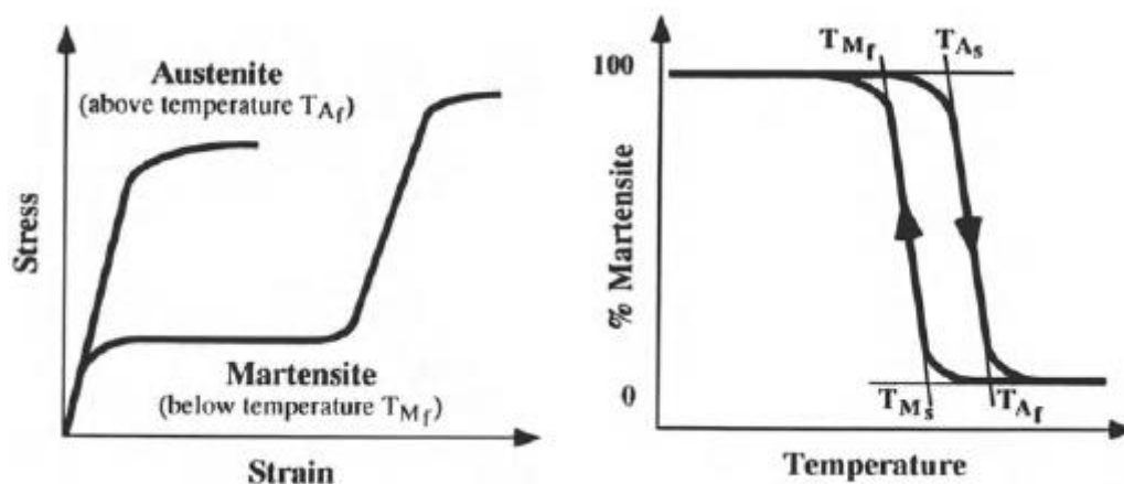
Fig.10. (a)Stress-Strain diagram and (b) the hysteresis curve of an SMA
