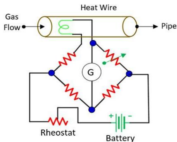
Fig. 25. Constant current method
