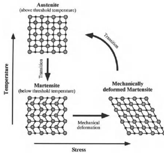
Fig.9. Schematic representation of SMA effect
