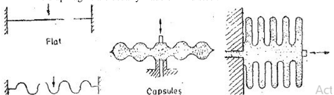
Fig.8. Types of Diaphragms
