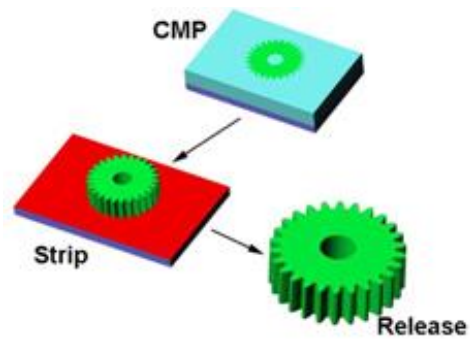
Fig.19. Strip, Release process in LIGA
