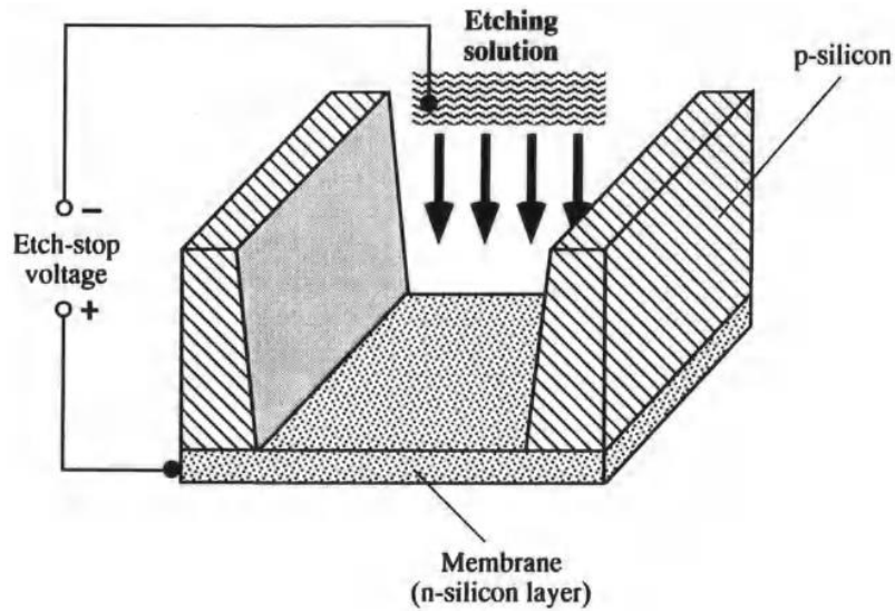
Fig.11. Membrane produced by the electrochemical etch-stop method
