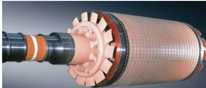
Fig.20. Wound rotor of a large induction motor
