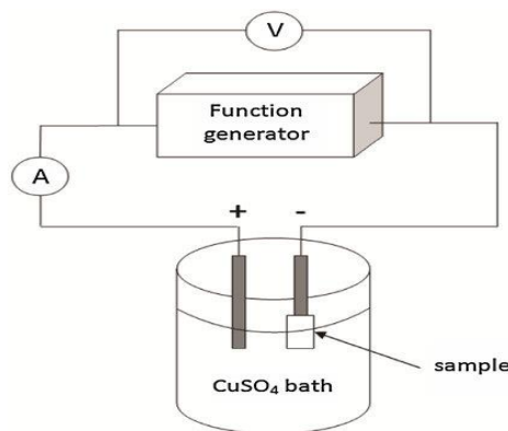
Fig.7. Example of copper Electro plating
