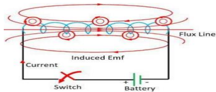
Fig. 4. Self Inductance
