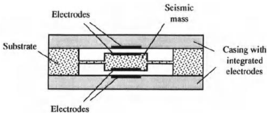
Fig.6. Capacitive measurement of accelerations
