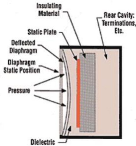
Fig.26. Capacitive pressure transducer Configuration
