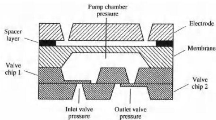
Fig.5. Electrostatic micro pump
