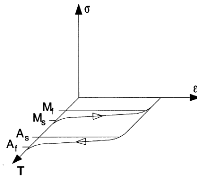
Fig.2 Strain – temperature characteristic for the two-way effect
