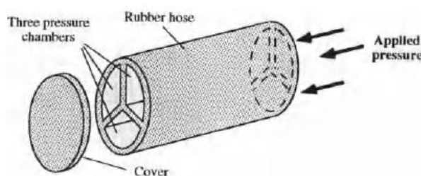
Fig.12. Principle of the pneumatically driven flexible micro actuator
