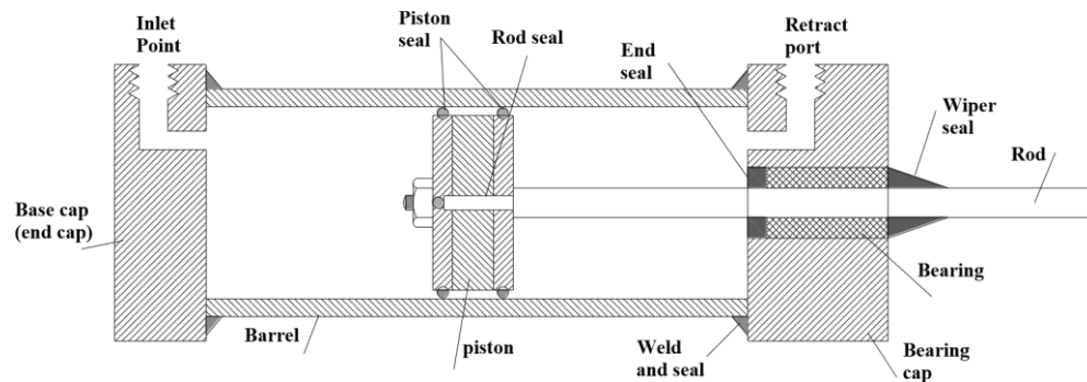
Fig 7 Construction features of double acting cylinder
