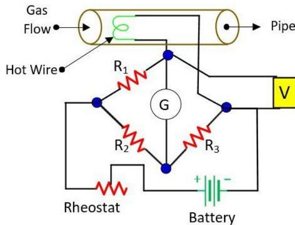
Fig. 26. Constant temperature method
