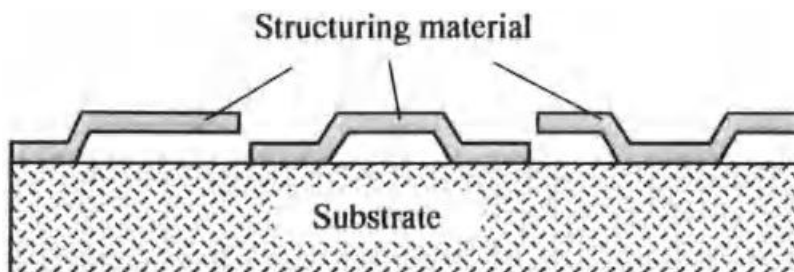
Fig. 14. Typical surface micromachining structures
