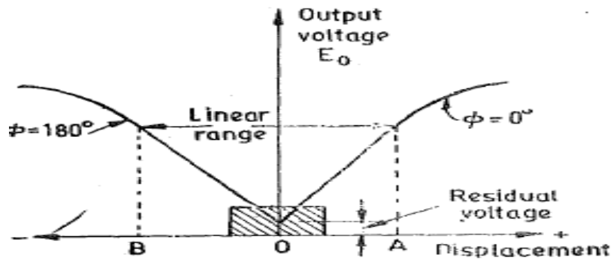
Fig.3. Variation in output voltage with linear displacement for an LVDT
