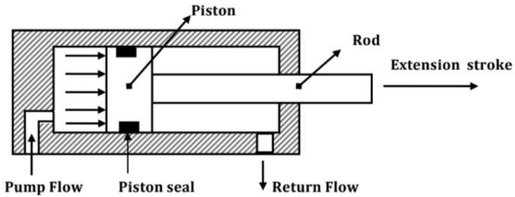
Fig. 8.a) Double acting Cylinder with piston rod on one side (Extension stroke)
