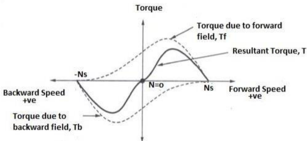
Fig.23. Torque-Speed Characteristics
