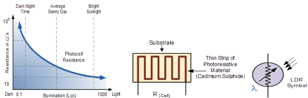
Fig.29. LDR characteristics and symbol
