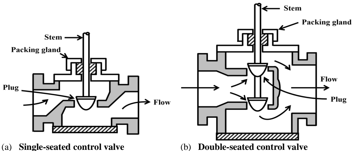
Fig. 12 Single-seated and double-seated valves
