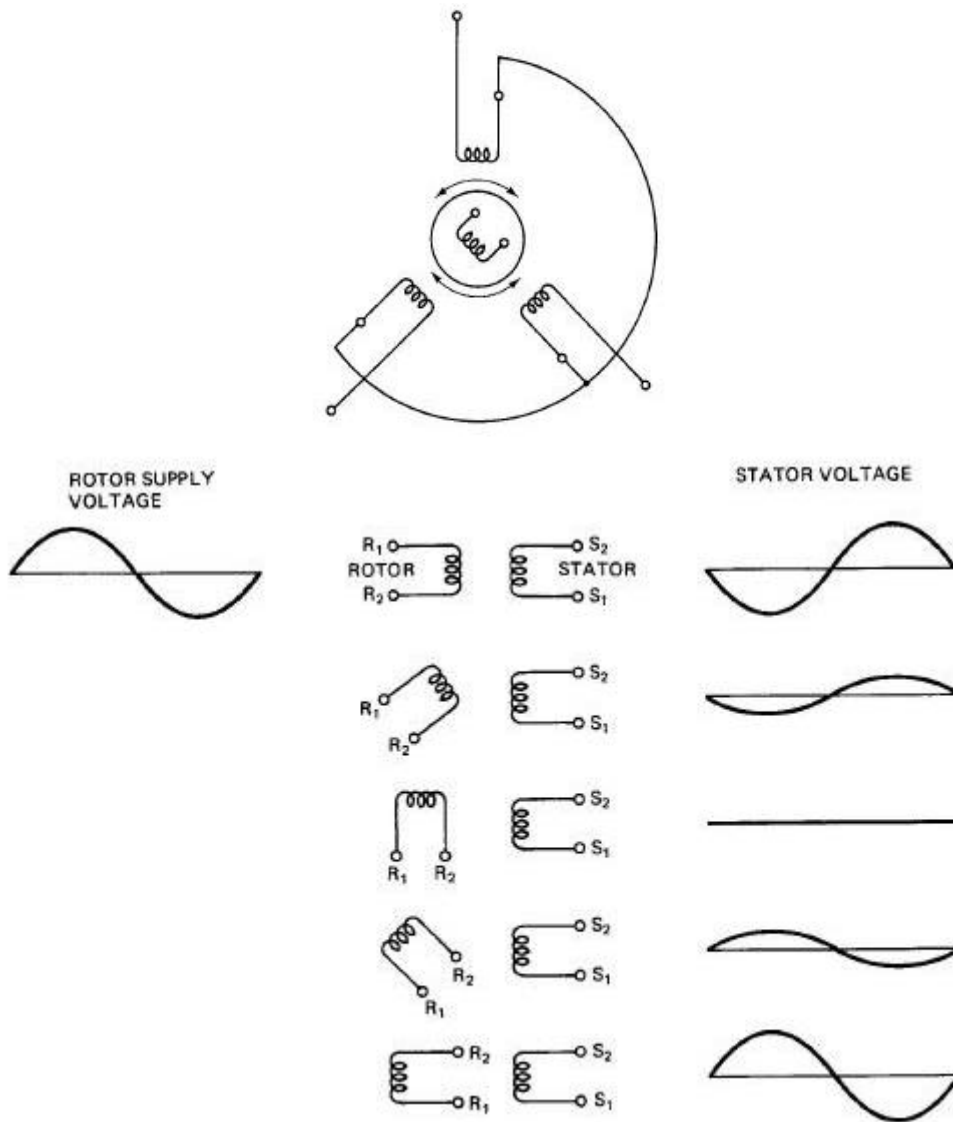
Fig.14. Synchros
