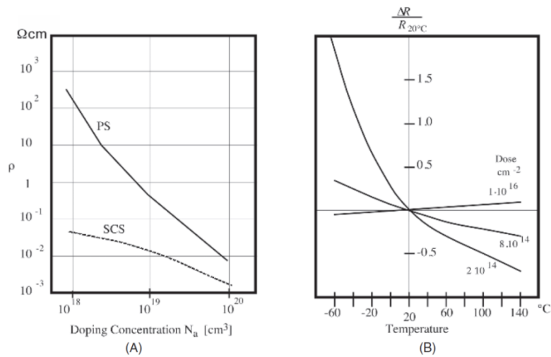
Fig.1. (A) Specific resistivity of boron-doped silicon, (B) temperature coefficient of resistivity of silicon for different doping concentrations.
