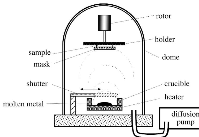
Fig.4. Deposition of a thin metal film in a vacuum chamber.
