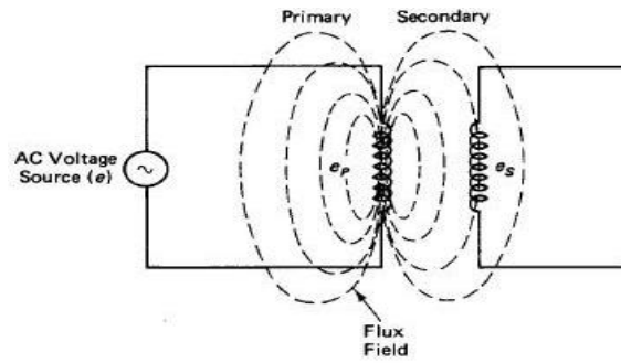
Fig.7. Transformer effect
