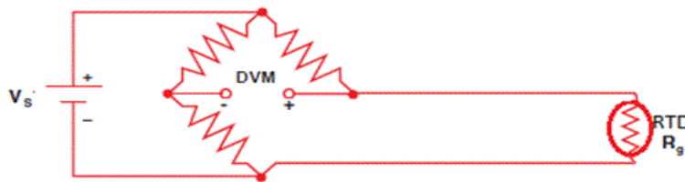
Fig. 19. Two wires RTD bridge
