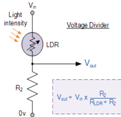
Fig.30. Application of LDR
