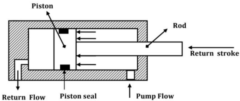
Fig. 8.b) Double acting Cylinder with piston rod on one side (Return stroke)
