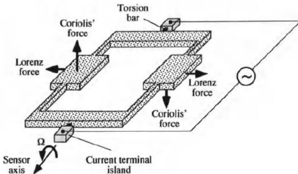
Fig.5. Operating principle of a rotational speed micro sensor
