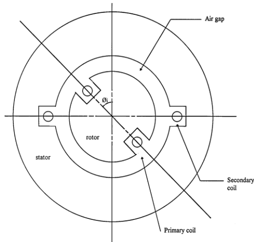
Fig.13. Inductance Potentiometer
