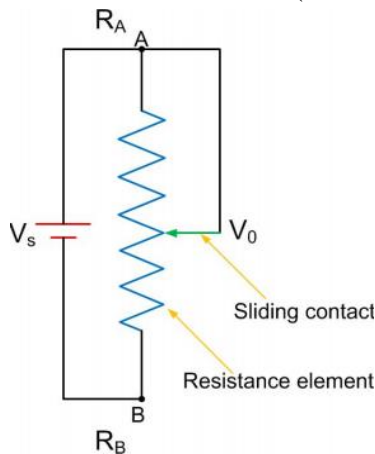
Fig. 12. Electric circuit of the potentiometer
