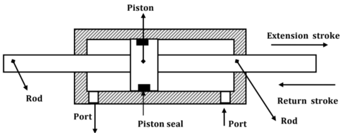
Fig.9 Double Acting Cylinder with piston rod on both side
