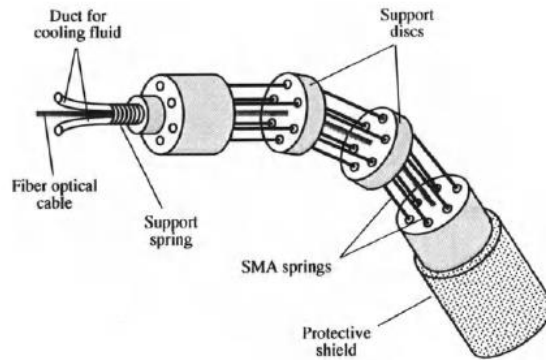
Fig.11. Active endoscope using SMA
