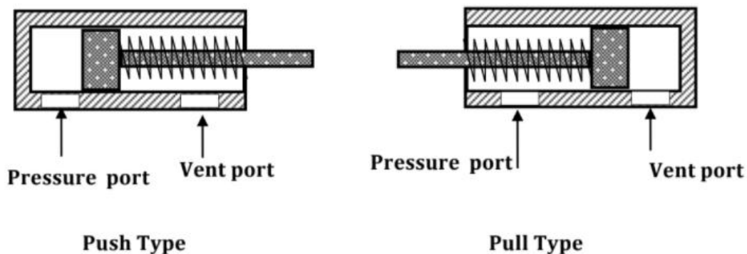
Fig.5 Push and Pull type Single Acting Cylinder
