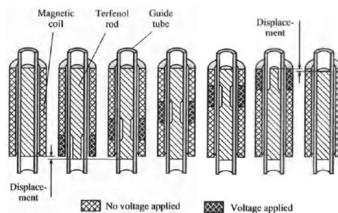
Fig.7. Magnetostrictive Micro actuators
