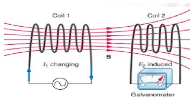
Fig.5. Mutual Inductance
