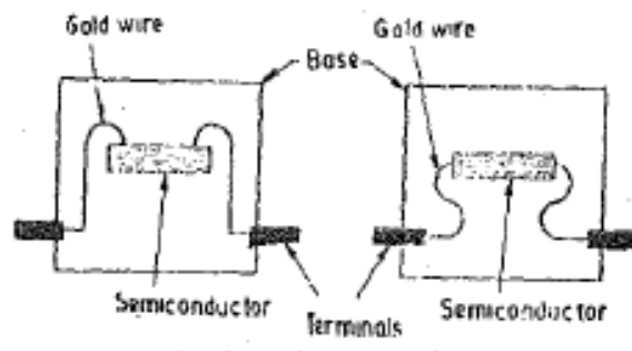
Fig. 15. Semiconductor strain gauge
