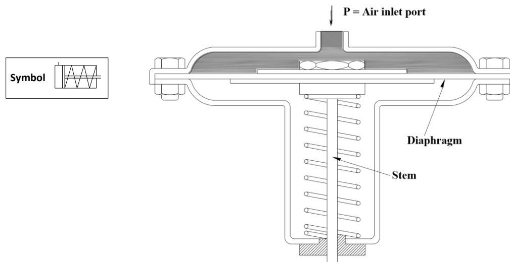
Fig.2 Construction features of diaphragm cylinder
