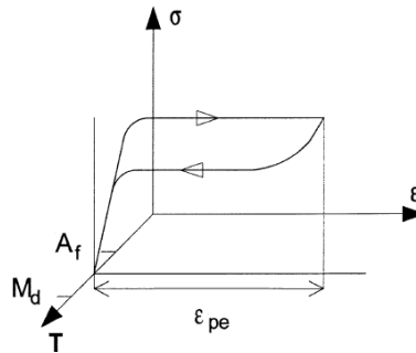
Fig.3 Stress- Strain characteristic for pseudo elasticity
