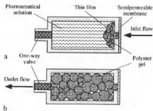
Fig.14. Polymer micro pump (a) Initial state (b) final state
