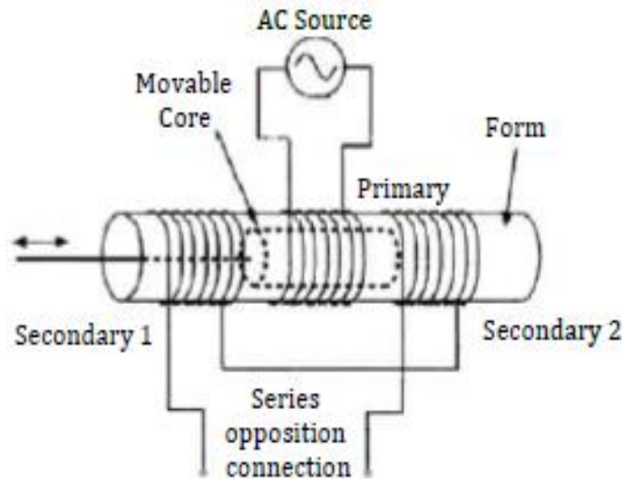
Fig.1. Construction of LVDT
