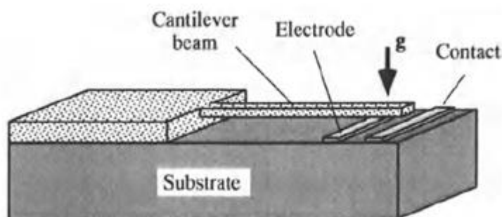
Fig. 8. Capacitive cantilever acceleration micro sensor
