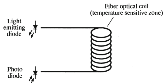
Fig.13. Fiber optic thermometer
