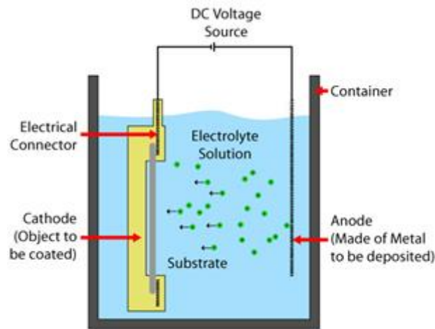
Fig.17. Electroplating
