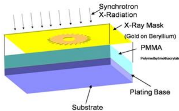
Fig.16. Micro gear using LIGA process
