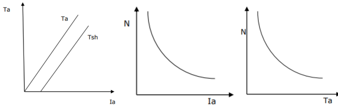
Fig.9. Series motor Characteristics
