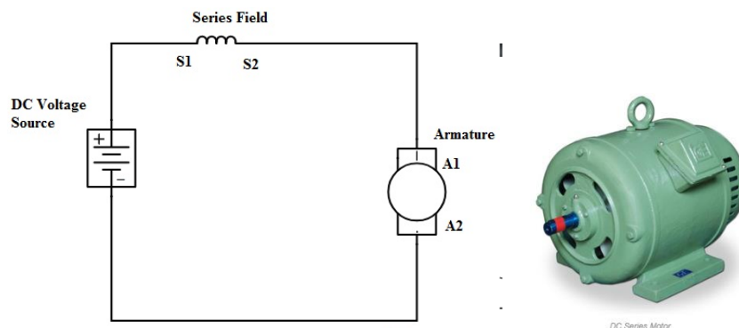
Fig.8.Series motor
