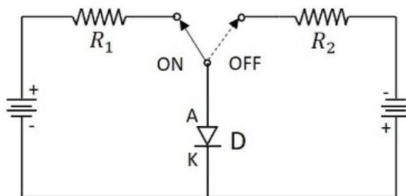
Fig.1. Diode as a Switch
