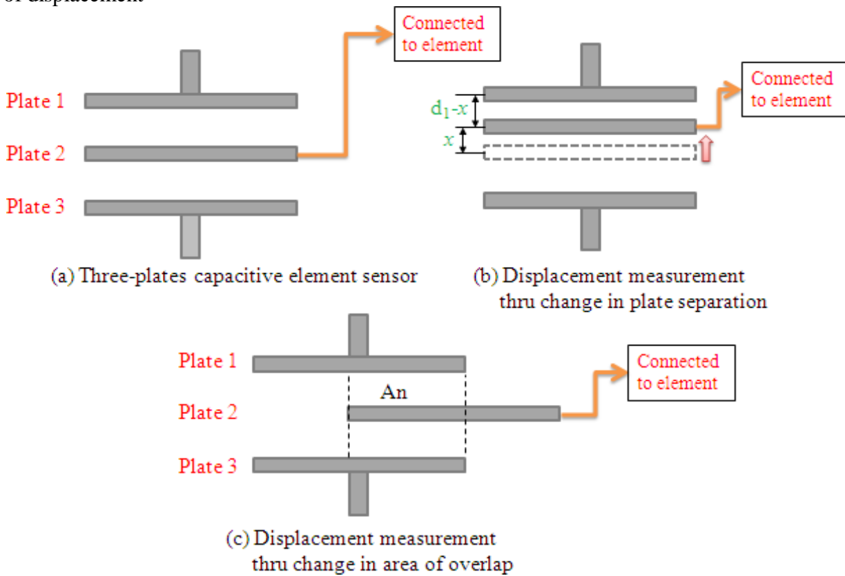
Fig.22. Capacitive transducer using principle of change in dielectric constant for measurement of displacement
