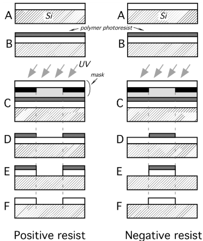
Fig.8. Photolithography
