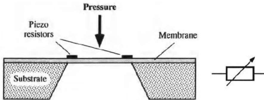
Fig. 1. Piezo resistive pressure sensor
