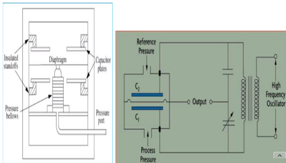
Fig.27. Application of Capacitive pressure transducer
